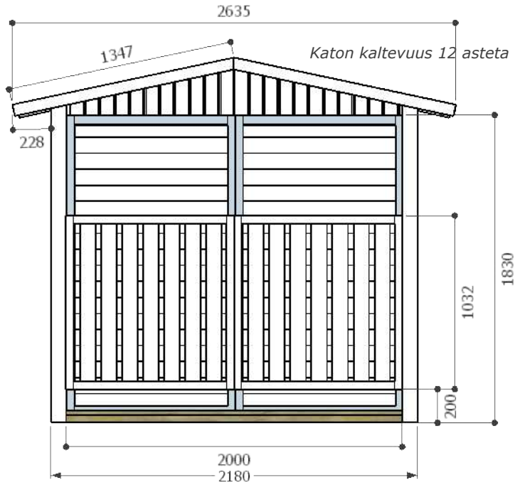
Rear view
